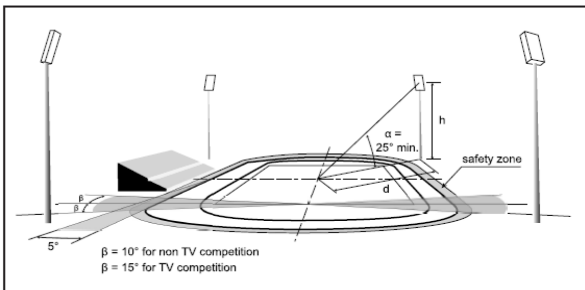
Figure 5.1.4.2 – Floodlights positioning
