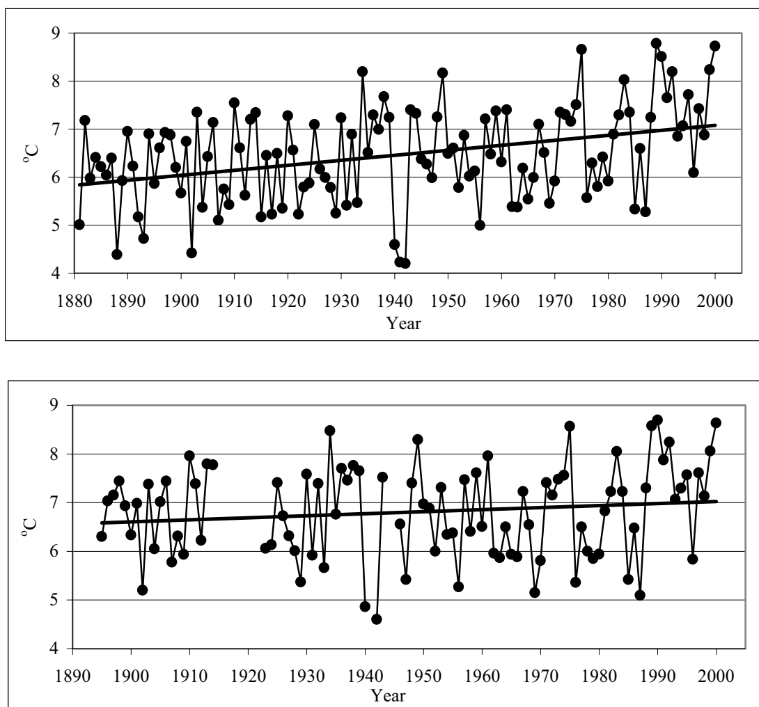
Figure 6.1. Annual mean temperature in Riga and Liepāja
