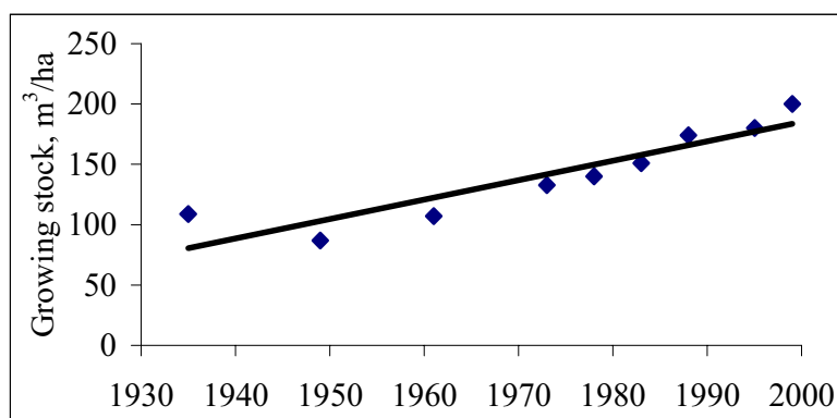
Figure 2.7. Average growing stock [31]
