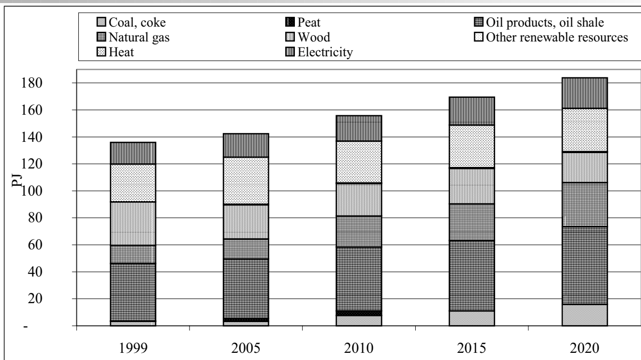
Figure 5.3. Final energy consumption in 1999-2020
