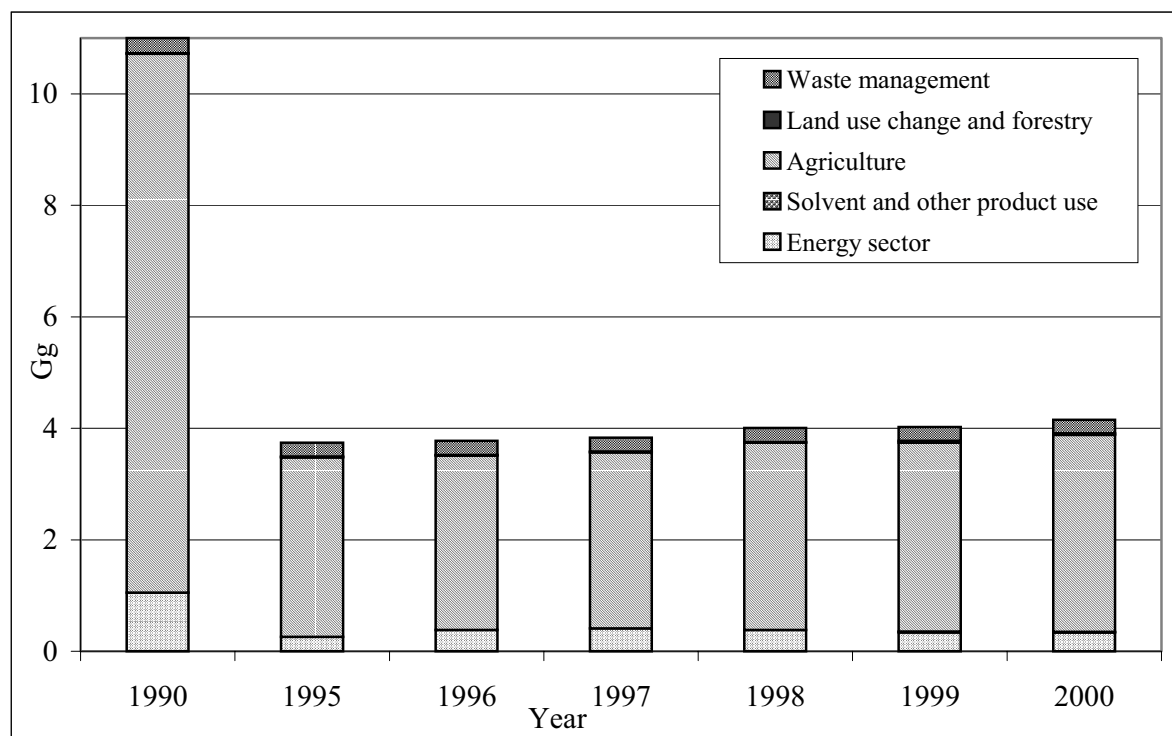
Figure 3.3. Total N 2 O emissions in 1990, 1995-2000
