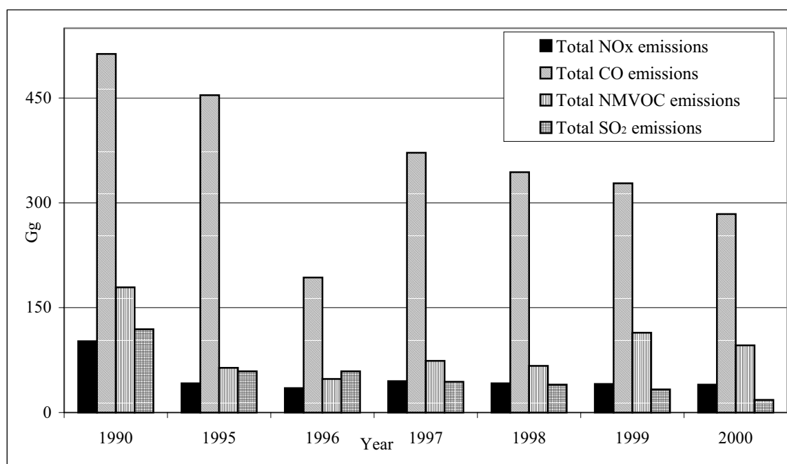
Figure 3.4. Indirect GHG and SO_2 emissions in 1990, 1995-2000
