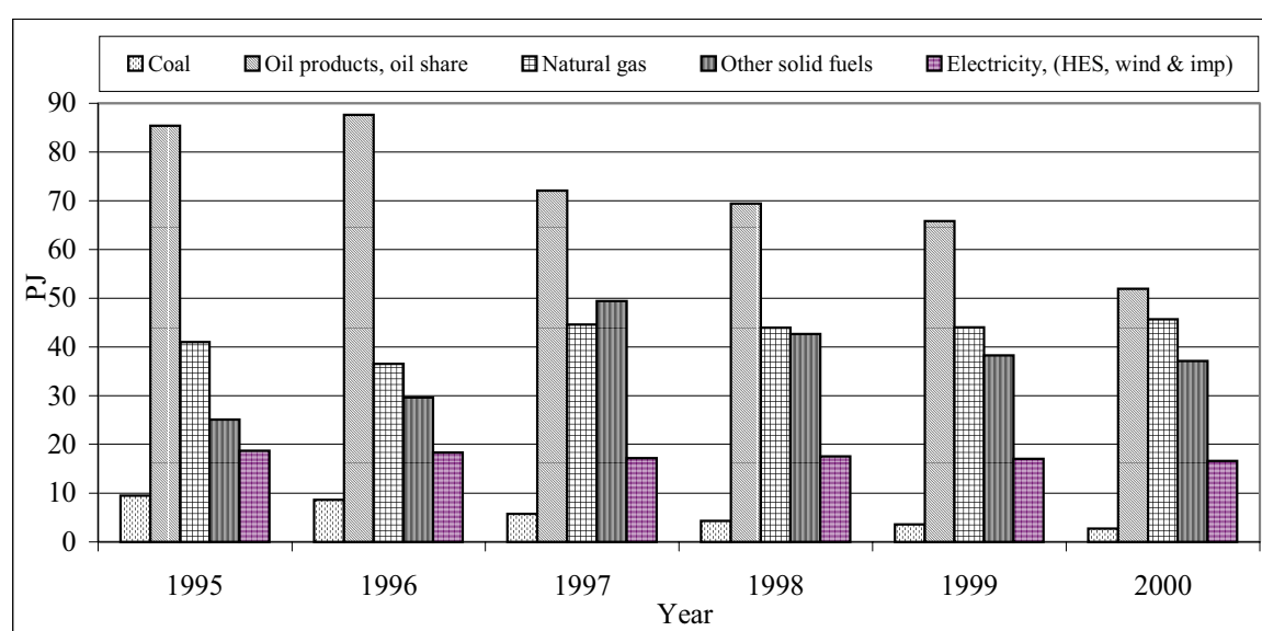
Figure 2.4. Consumption of primary energy resources, PJ [20, 78]
