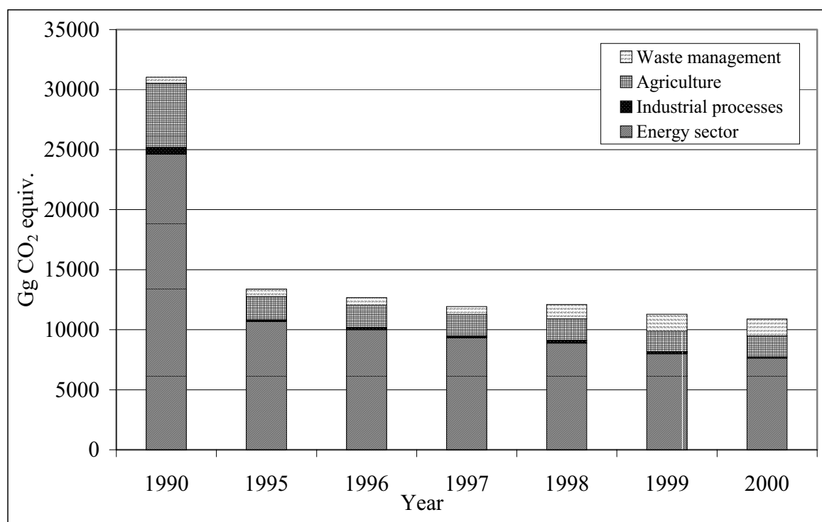
Figure 3.6. Share of sectors in aggregated GHG emissions in 1990, 1995-2000
