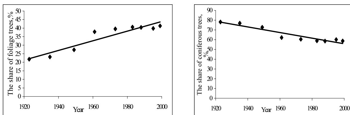
Figure 6.3. Dynamics of foliage and coniferous trees [31]
